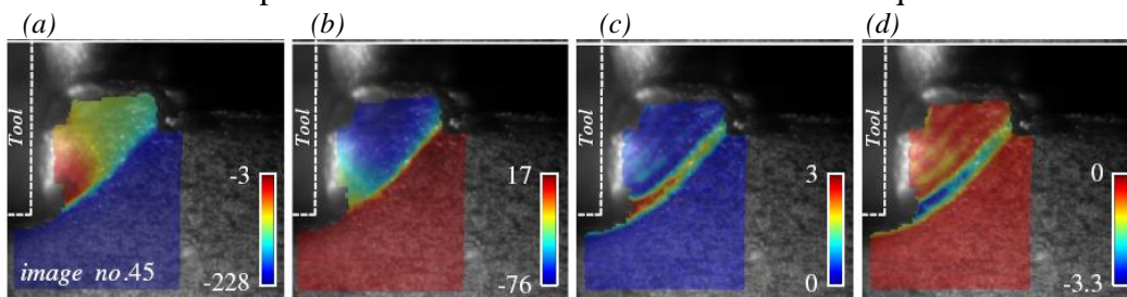
Figure 1 : (a) Horizontal displacement (in \mu m ). (b) Vertical displacement (in \mu m ). (c) Major strain. (d) Minor strain during the machining of the titanium alloys Ti64 ( a_p = 0.25 mm ; V_c = 6 m/min ) [1]
